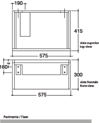
9107 BUDDY mobile sospeso 60 cm BUDDY wall-mounted cabinet 60 cm
