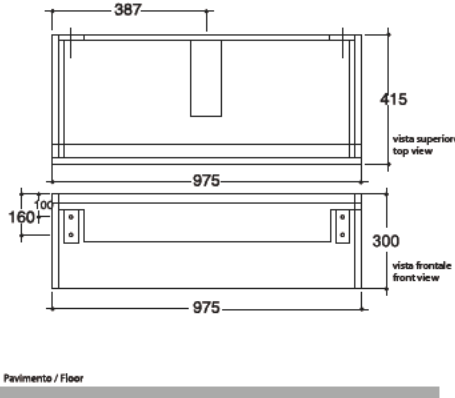
9109 BUDDY mobile sospeso 100 cm BUDDY wall-mounted cabinet 100 cm
