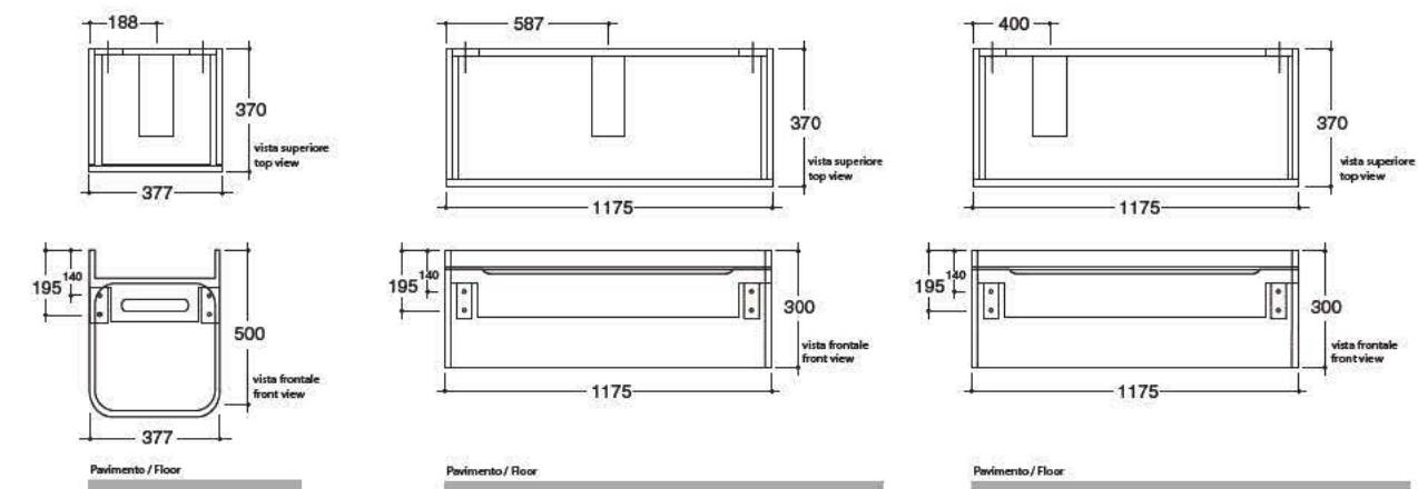
9110 INKA mobile sospeso 40 cm INKA wall-mounted cabinet 40 cm
