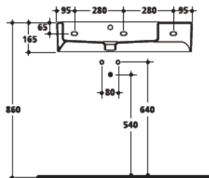
3143 Lavabo 75x42 cm sospeso o appoggio monoforo vasca asimmetrica One hole wall hung or freestanding asymmetrical washbasin 75x42 cm
