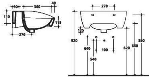
3342 Lavabo 60x55 sospeso monoforo One hole wall hung washbasin 60x55
