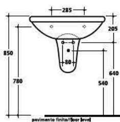
2355/2366 - 2375 Lavabo 55/66 cm su semicolonna Washbasin 55/66 cm on half pedestal
