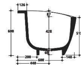
3350 Vasca 170x80x60 in Pietraluce Pietraluce bath-tub 170x80x60
