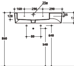
3243 Lavabo 75x43 cm sospeso o appoggio monoforo vasca asimmetrica One hole wall hung or freestanding asymmetrical washbasin 75x43 cm
