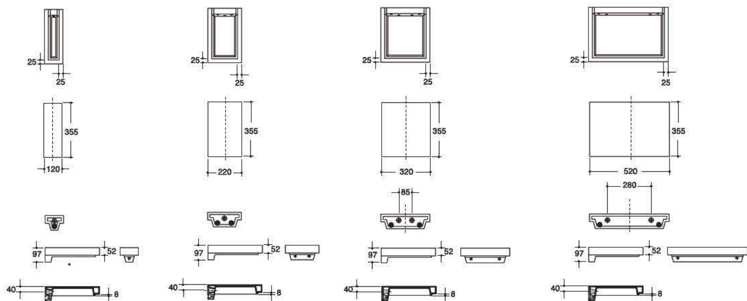
3415 INKA Piano in ceramica 12x35,5 INKA Ceramic counter 12x35,5
