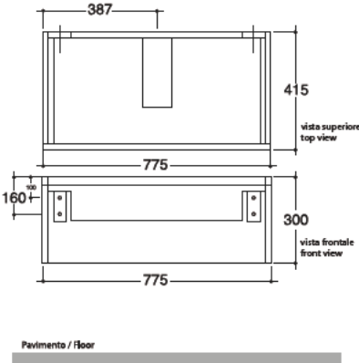
9108 BUDDY mobile sospeso 80 cm BUDDY wall-mounted cabinet 80 cm
