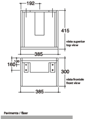
9106 BUDDY mobile sospeso 40 cm BUDDY wall-mounted cabinet 40 cm
