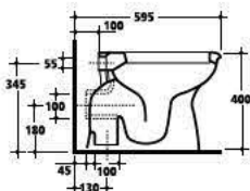
2310 - 2311 Vaso scarico "S" - "P" We pan wall - floor outlet
