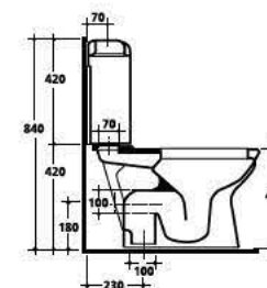
2312 - 2313 Vaso monoblocco scarico "S" - "P" Closed coupled wc pan floor - wall outlet
