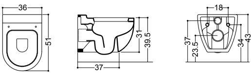
ART. 14010 vaso sospeso wall-hung wc
