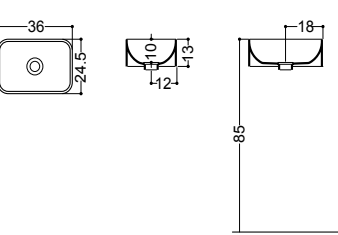
ART. WS102 01S lavabo da appoggio senza piano rubinetteria 01S overtop basin without tap hole
