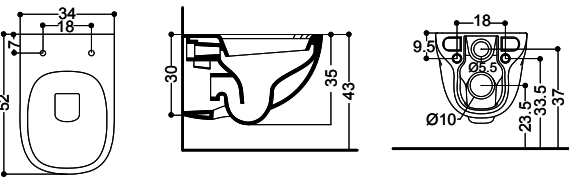
ART. 30060 vaso sospeso NORIM wall-hung wc NORIM
