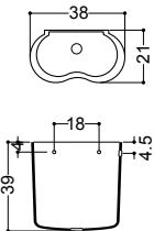
ART. 06050 cassetta alta high level cistern
