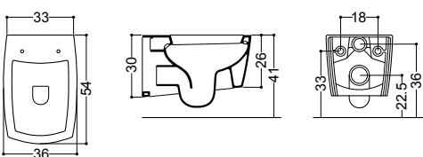
ART. 29010 vaso sospeso wall-hung wc
